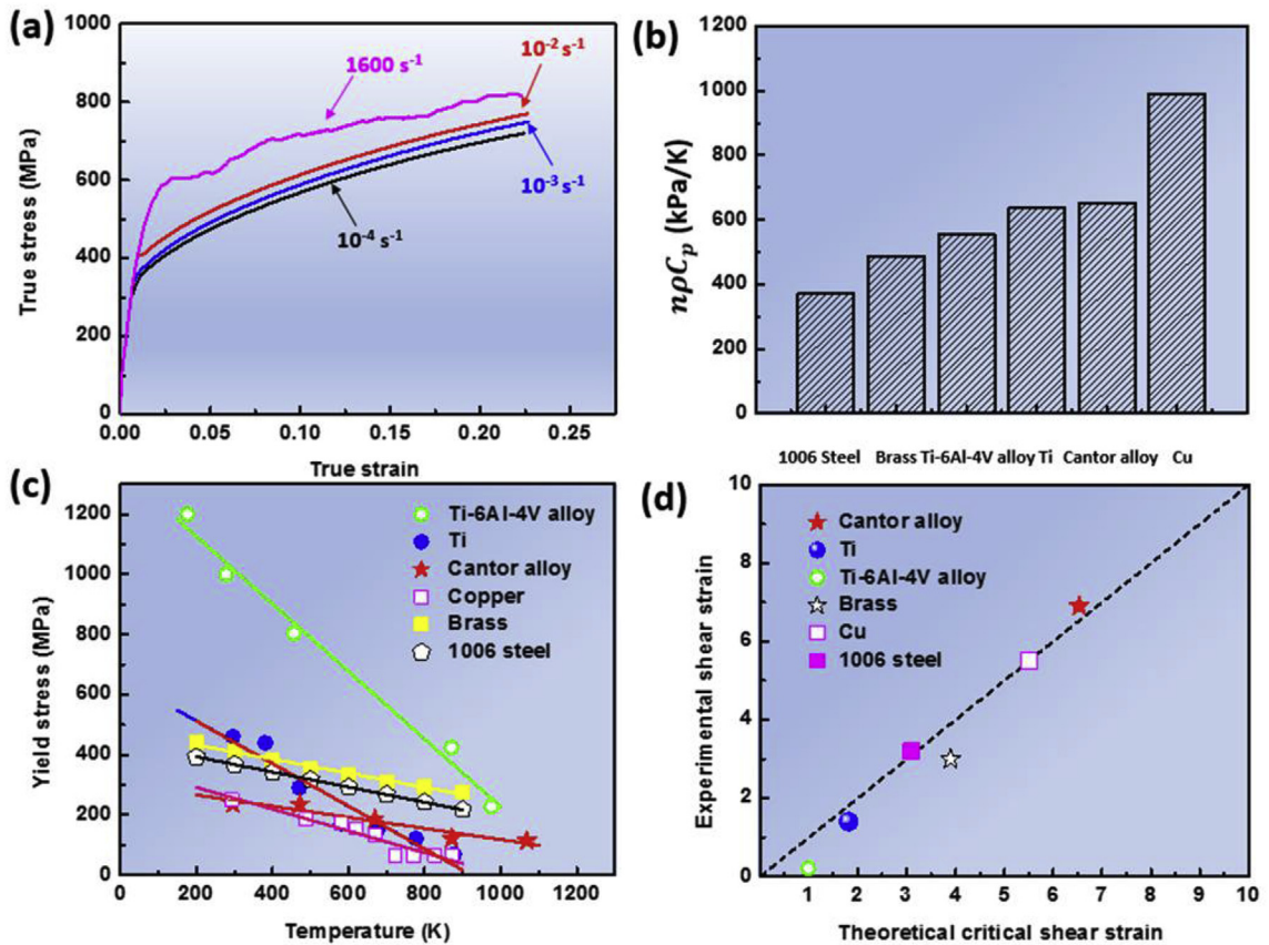
Fig. 4. (a) Mechanical response of the Cantor alloy under different strain-rates; (b) the value of \rho C_p n for pure Ti [32], Ti-6Al-4V alloy [33], 1006-Steel [34], Copper [34], Brass [34] and the Cantor alloy; (c) thermal-softening effect of different materials [22,32,33,35,36]; (d) experimental and predicted critical shear strain for shear localization [34,36].
