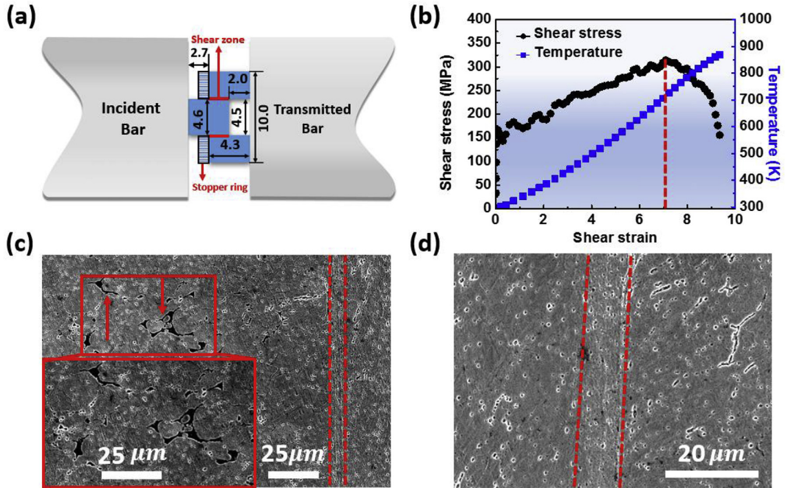
Fig. 3. (a) Schematic drawing of dynamic loading of the hat-shaped specimen with the stopper ring (in mm) by the split-Hopkinson pressure bar; (b) shear stress, shear strain and temperature evolution of the shear band; (c) scanning electron microscope (SEM) image showing separation of particles near the shear band; (d) SEM image of the shear band.
